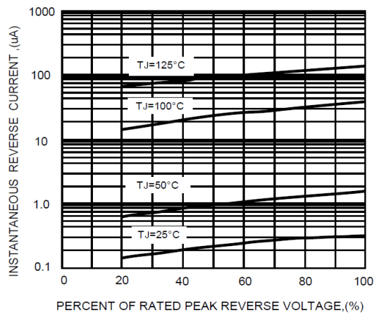
FIG.5-TYPICAL REVERSE CHARACTERISTICS
