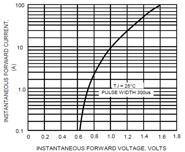
FIG.4-TYPICAL FORWARD CHARACTERISTICS
