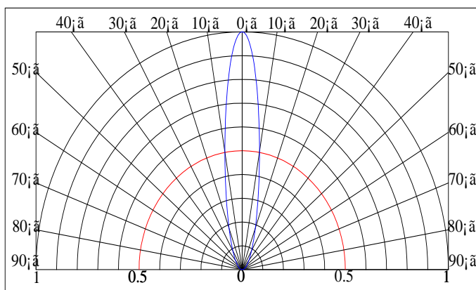
Radiation Diagram
