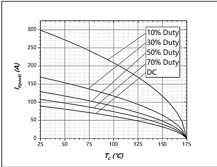
Figure 3. Current Derating
