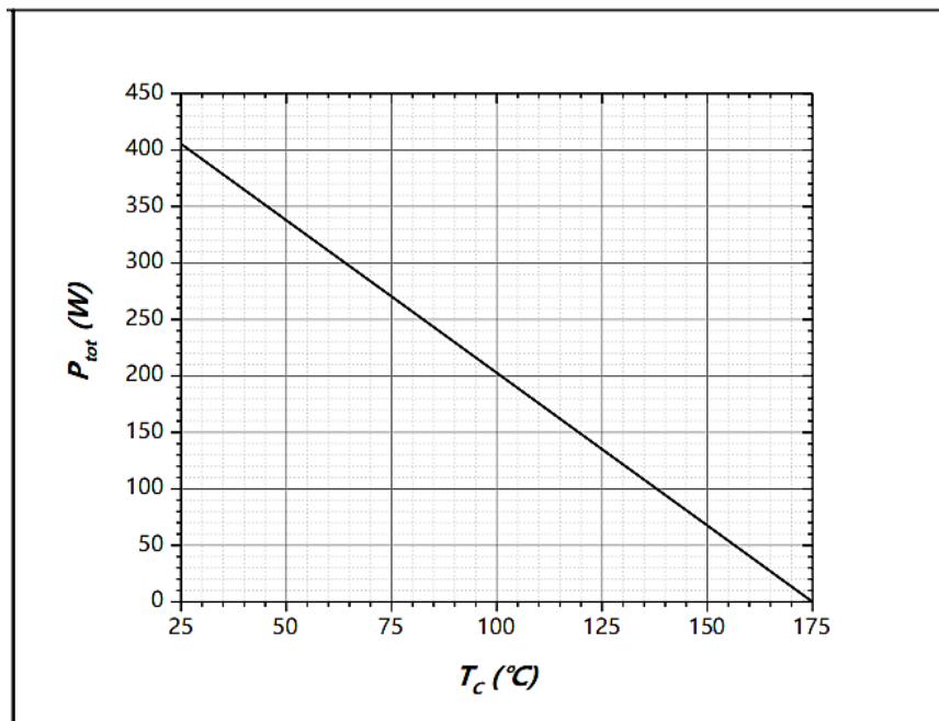
Figure 4. Power Derating
