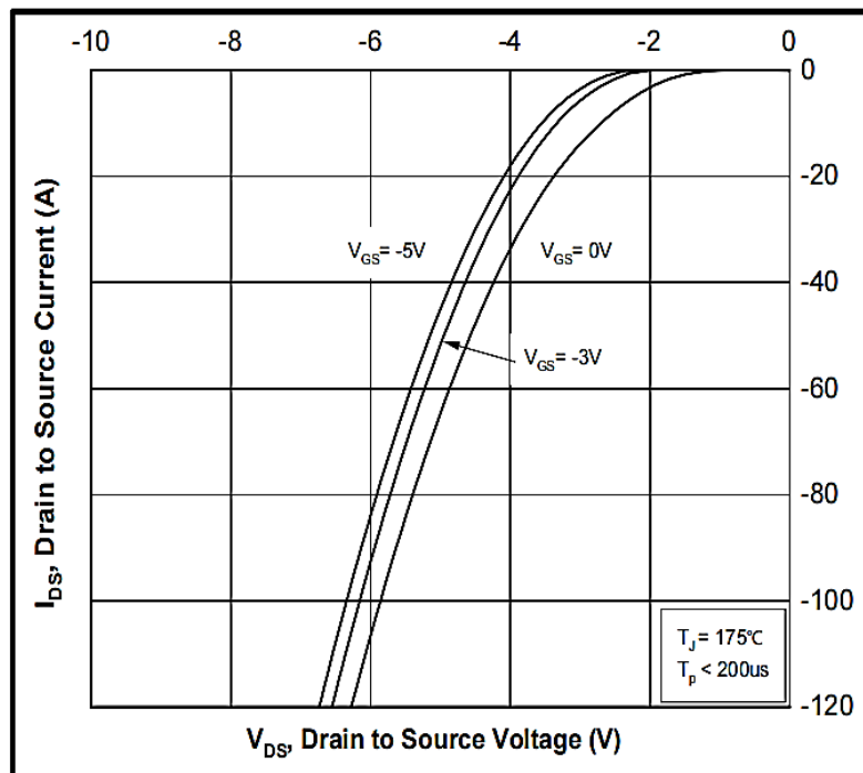
Figure 10. Body Diode Characteristic at 175°C
