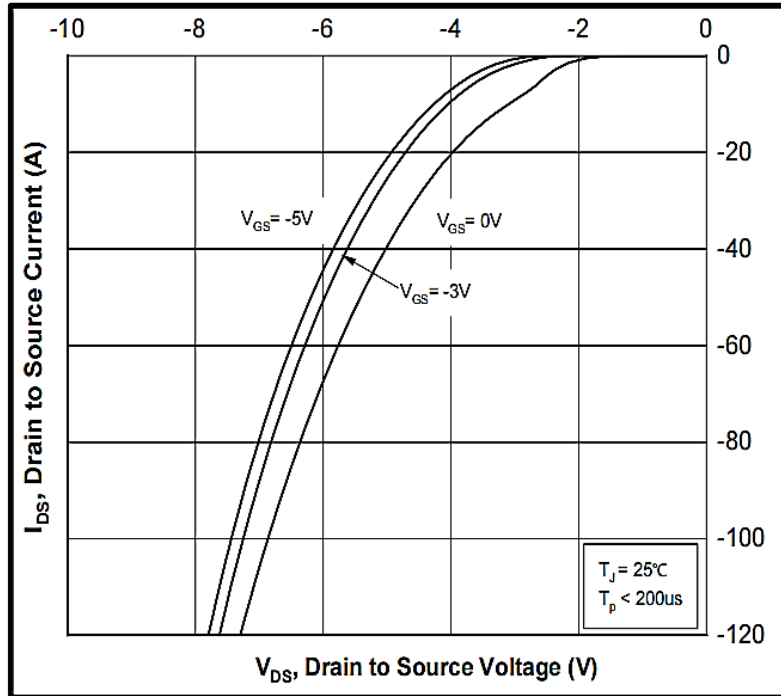
Figure 9. Body Diode Characteristic at 25°C
