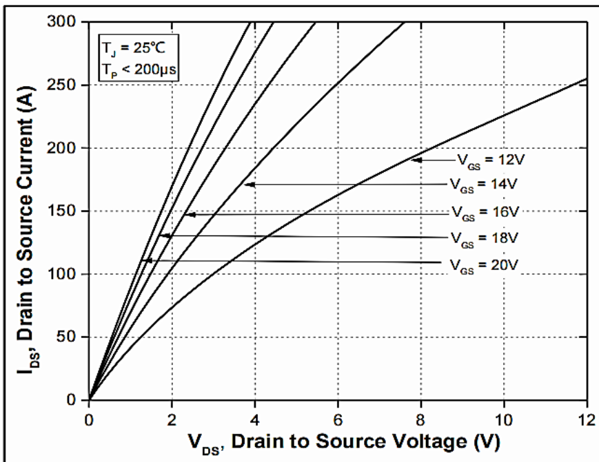
Figure 2. Output Characteristics T_J = 25^\circ\text{C}
