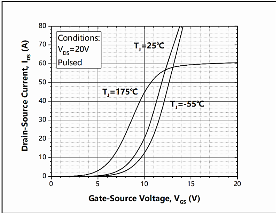
Figure 7. Transfer Characteristic for Various Junction Temperatures
