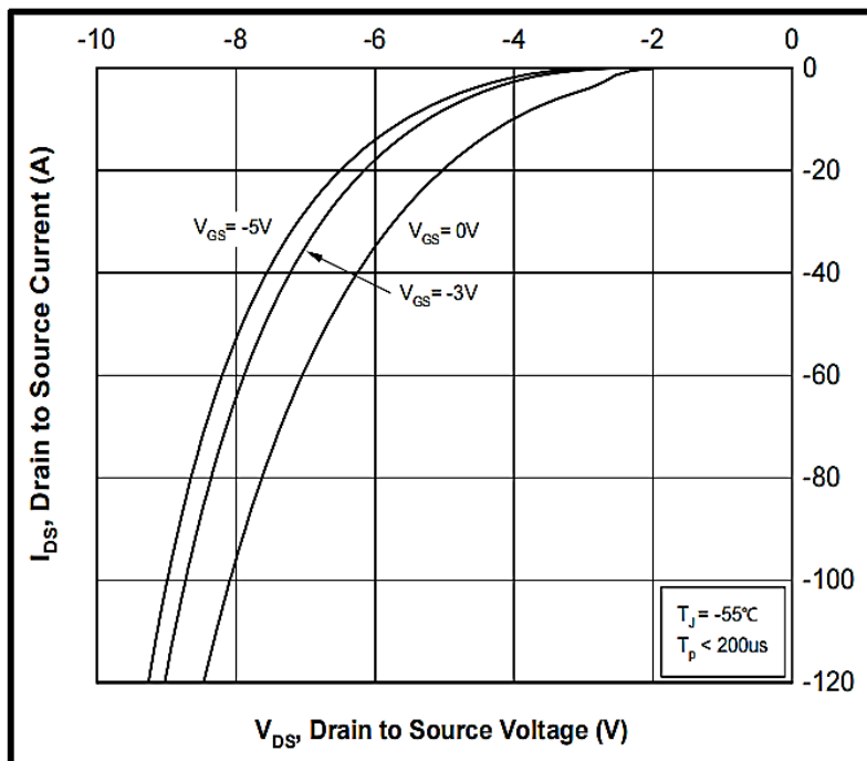
Figure 8. Body Diode Characteristic at -55°C
