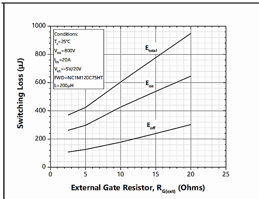
Figure 24. Clamped Inductive Switching Energy vs. R_{G(ext)}
