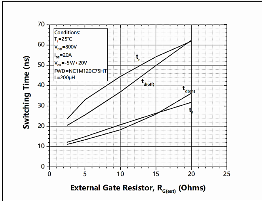
Figure 25. Switching Time vs. R_{G(\text{ext})}
