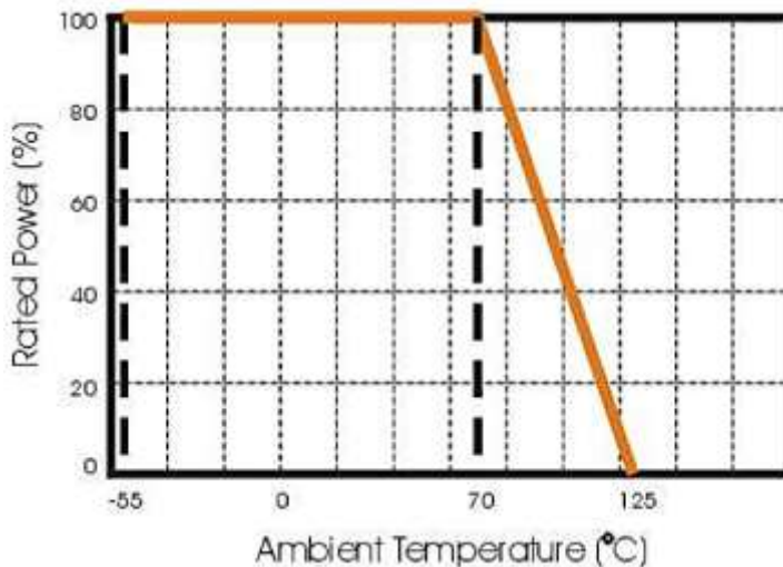
Fig 1 Maximum dissipation in percentage of rated power as a function of the ambient temperature for CR01
