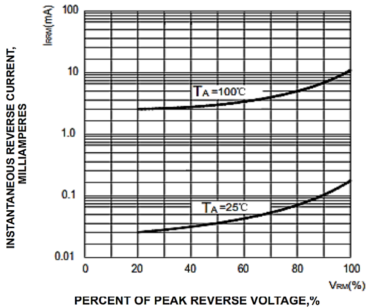
FIG. 4-TYPICAL REVERSE LEAKAGE CHARACTERISTICS
