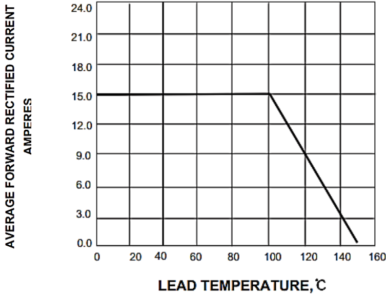
FIG. 1- DERATING CURVE OUTPUT RECTIFIED CURRENT
