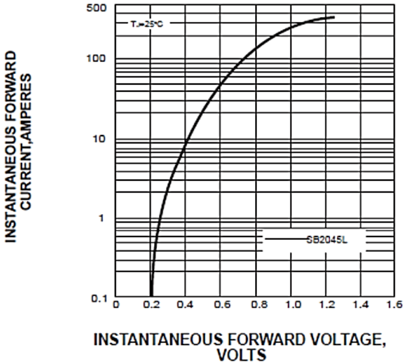
FIG. 3-TYPICAL FORWARD VOLTAGE CHARACTERISTICS
