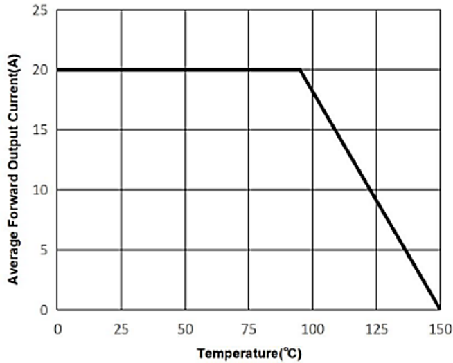
FIG.1: Forward Output Current Derating Curve
