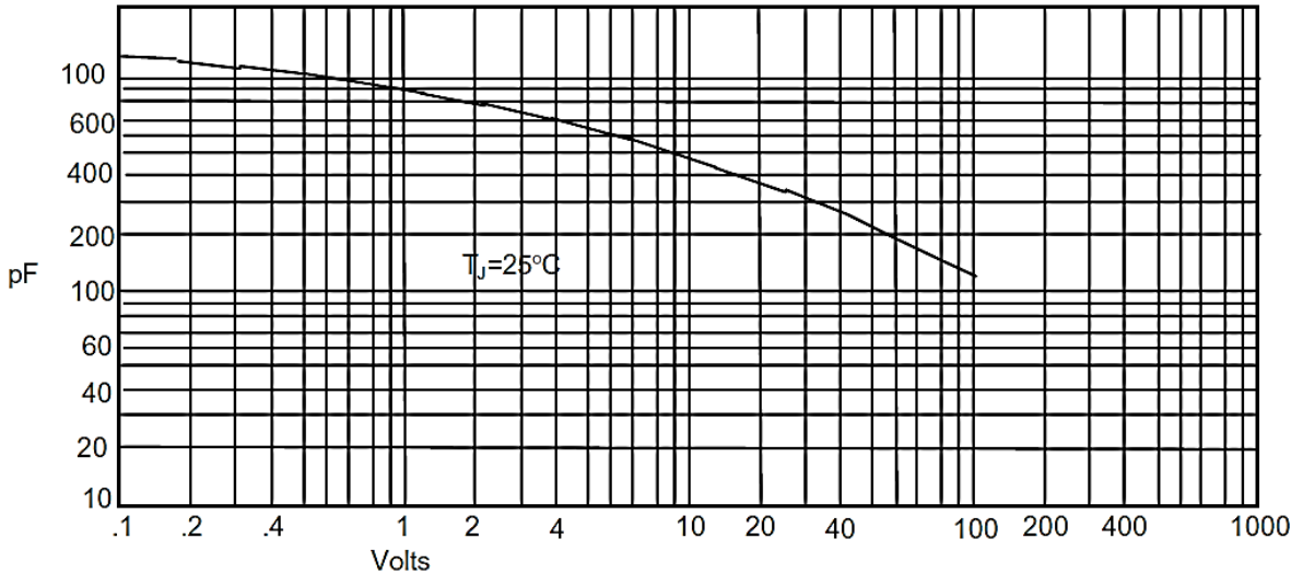
Figure 3 Junction Capacitance
