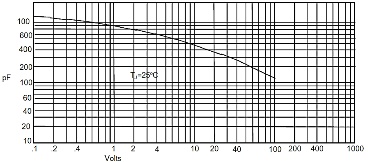
Figure 3 Junction Capacitance
