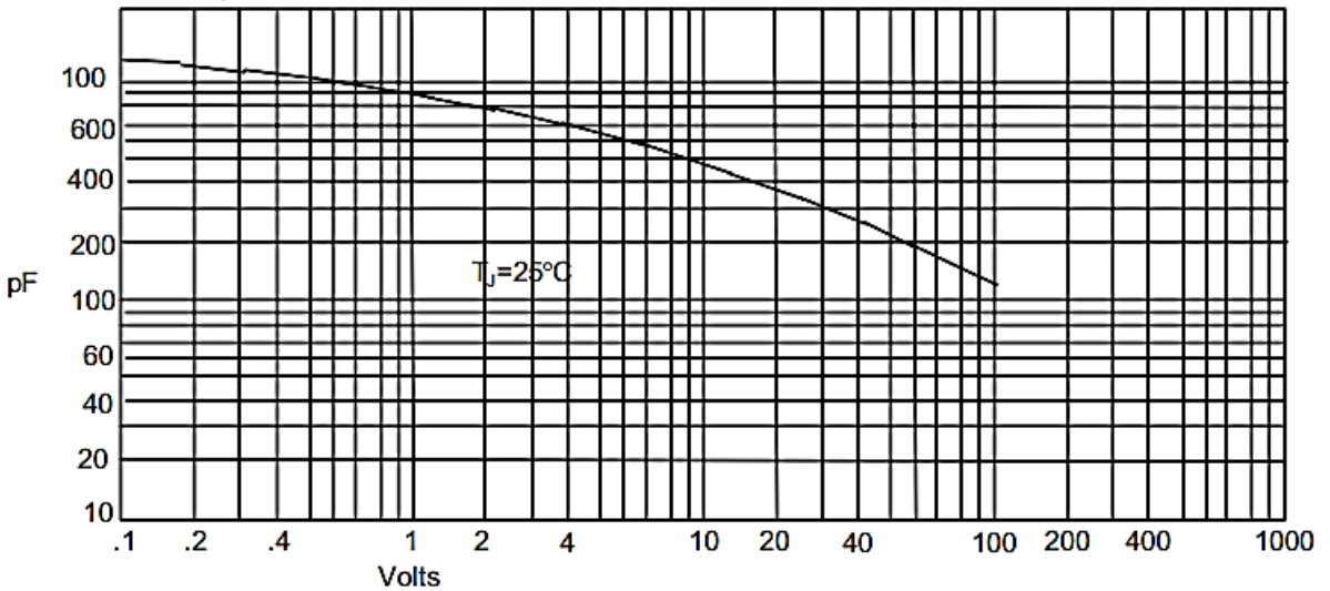
Junction Capacitance - pF versus Reverse Voltage - Volts
