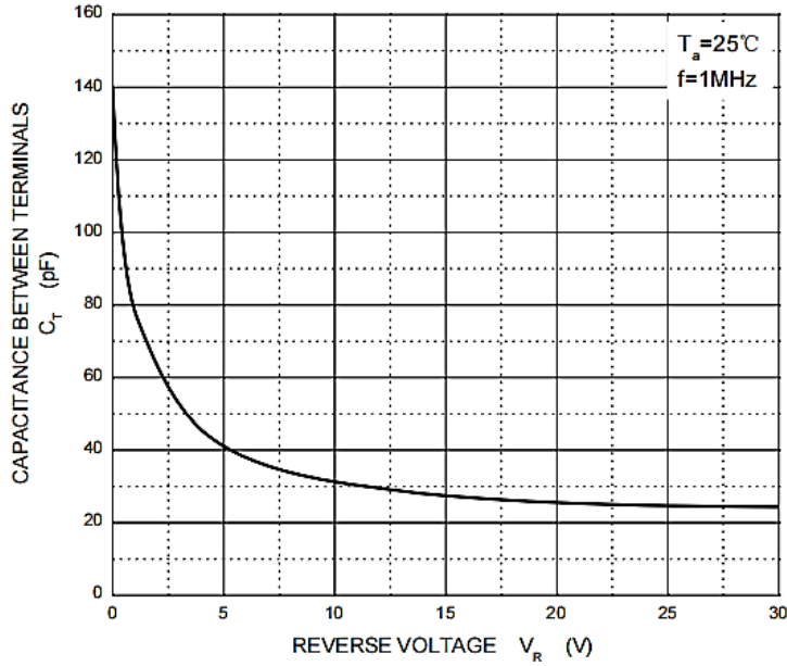
Capacitance Characteristics
