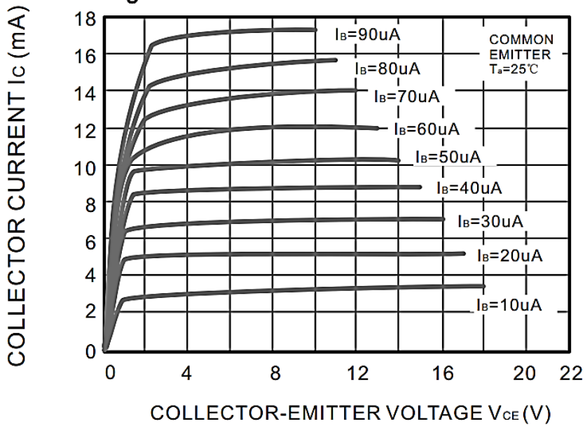
Fig.1 Static characteristics
