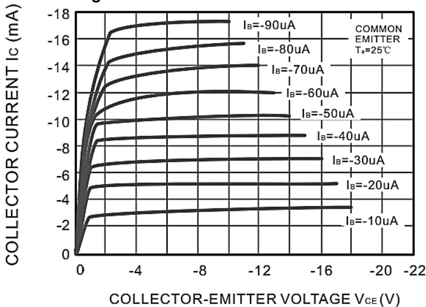
Fig.1 Static characteristics
