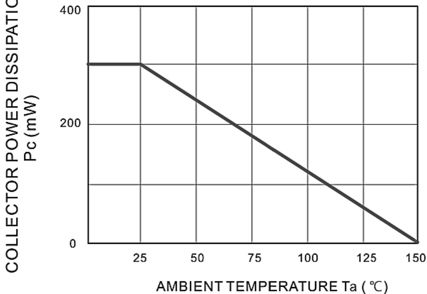
Fig.2 P_c — T_a
