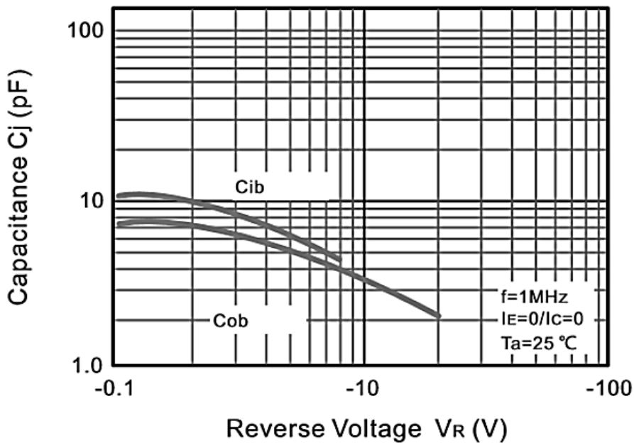
Fig.8 C_{ob}/C_{ib} - V_{CB}/V_{EB}
