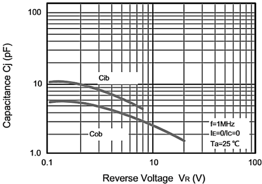
Fig.8 C_{ob}/C_{ib} - V_{CB}/V_{EB}
