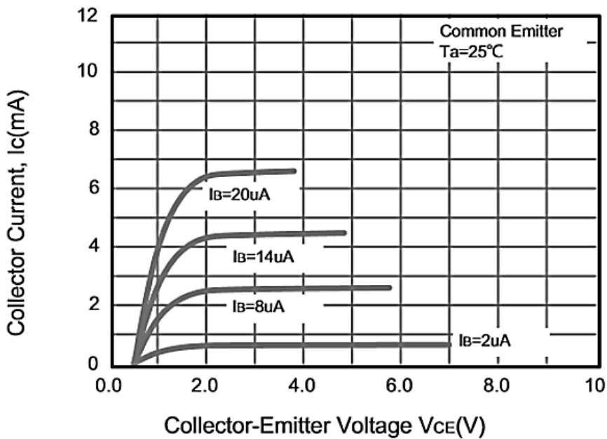
Fig.2 Static characteristics
