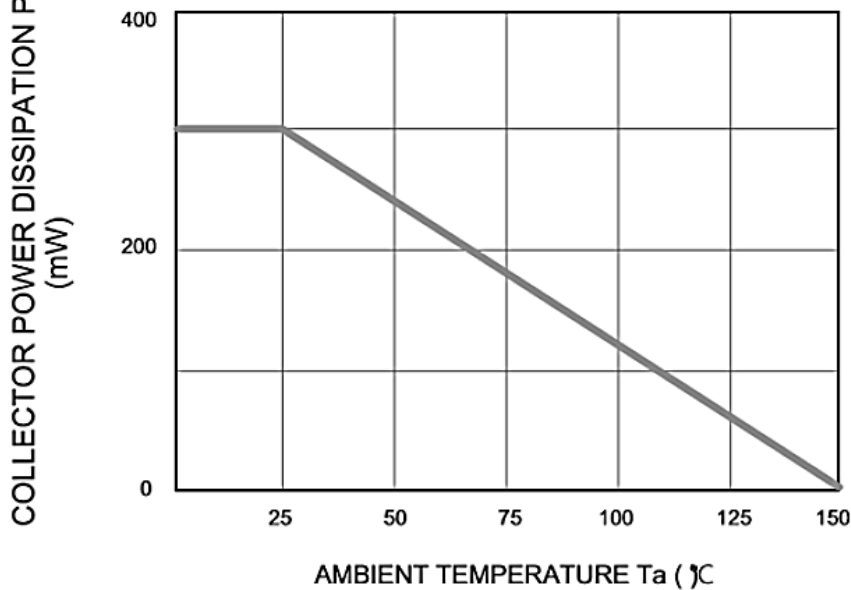
Fig.2 P_c — T_a
