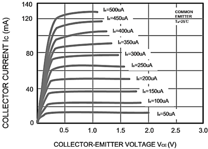
Fig.1 Static characteristics
