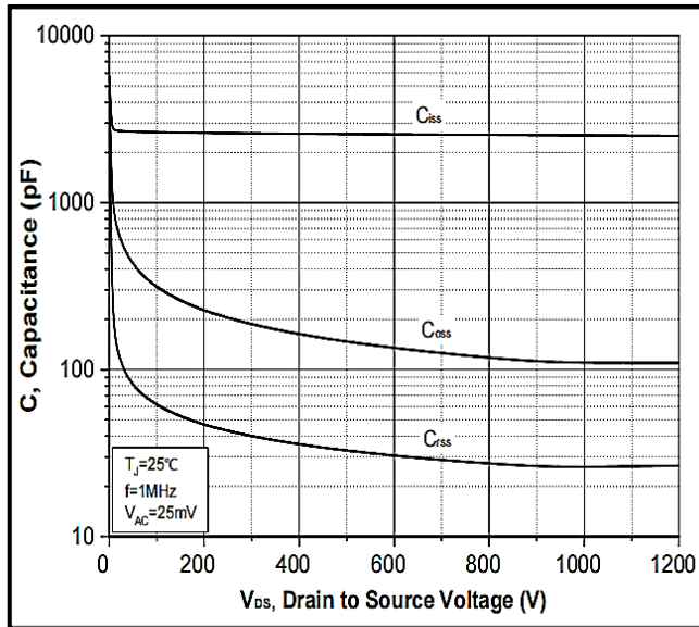
Figure 17. Capacitances vs. Drain-Source Voltage
