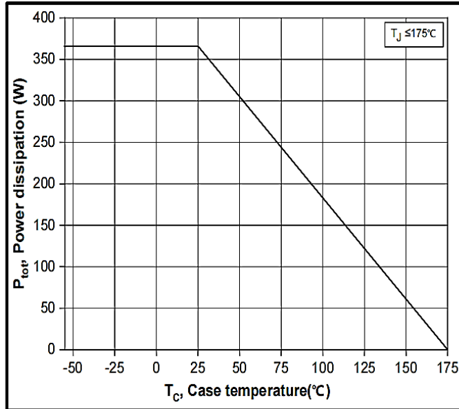
Figure 19. Maximum Power Dissipation Derating vs. Case Temperature
