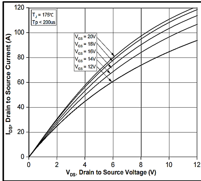
Figure 3. Output Characteristics T_J=175^\circ\text{C}
