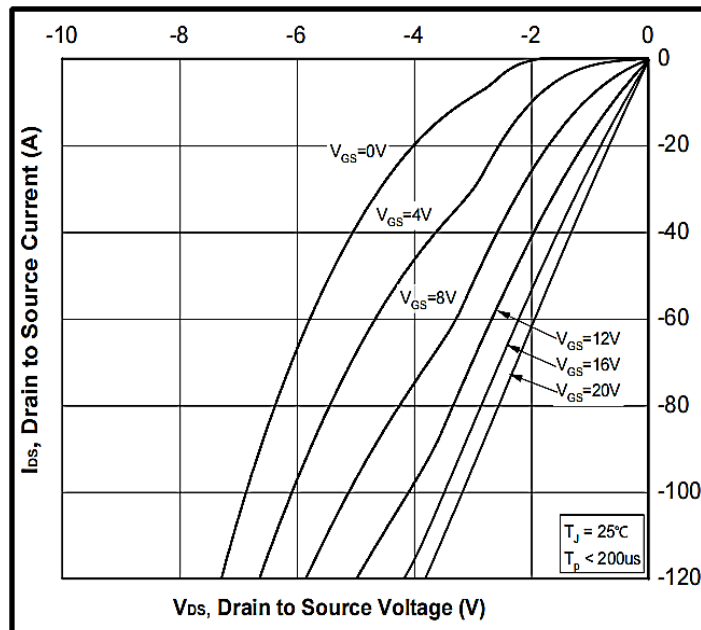
Figure 14. 3 rd Quadrant Characteristic at 25^\circ\text{C}
