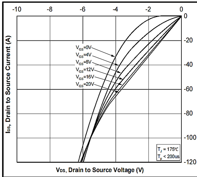
Figure 15. 3 rd Quadrant Characteristic at 175°C
