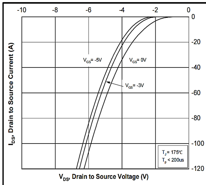
Figure 10. Body Diode Characteristic at 175°C
