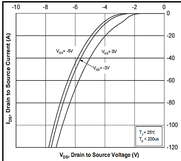
Figure 9. Body Diode Characteristic at 25°C
