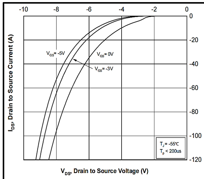
Figure 8. Body Diode Characteristic at -55^\circ\text{C}
