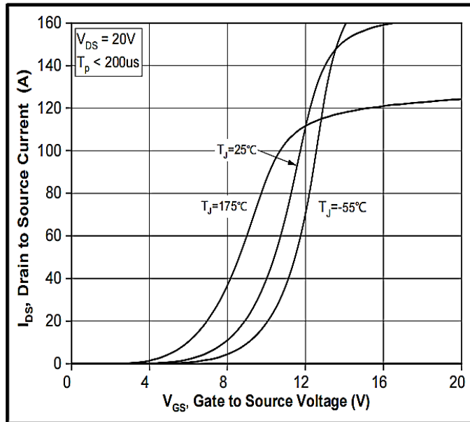
Figure 7. Transfer Characteristic for Various Junction Temperatures
