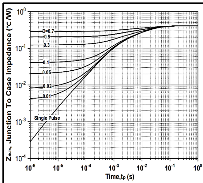
Figure 20. Transient Thermal Impedance (Junction - Case)
