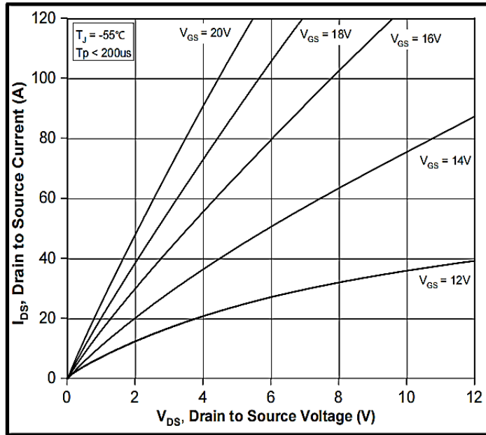
Figure 1. Output Characteristics T_J = -55^\circ\text{C}
