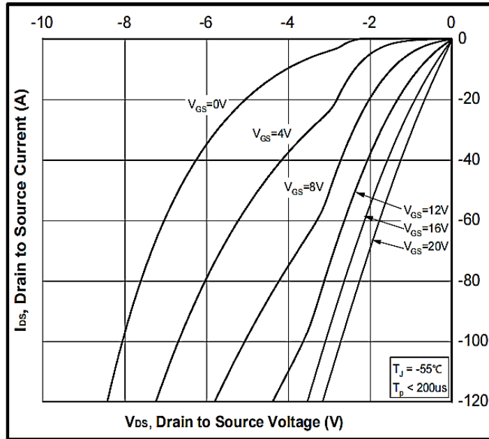
Figure 13. 3 rd Quadrant Characteristic at -55^\circ\text{C}
