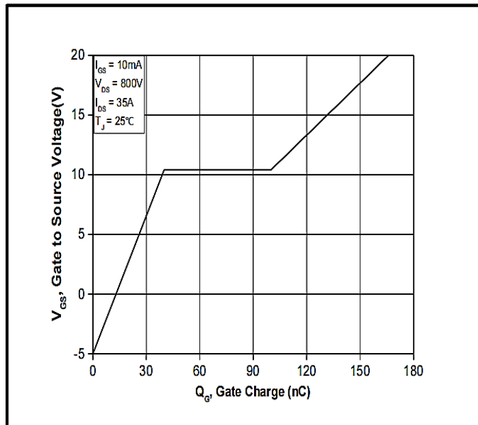
Figure 12. Gate Charge Characteristics
