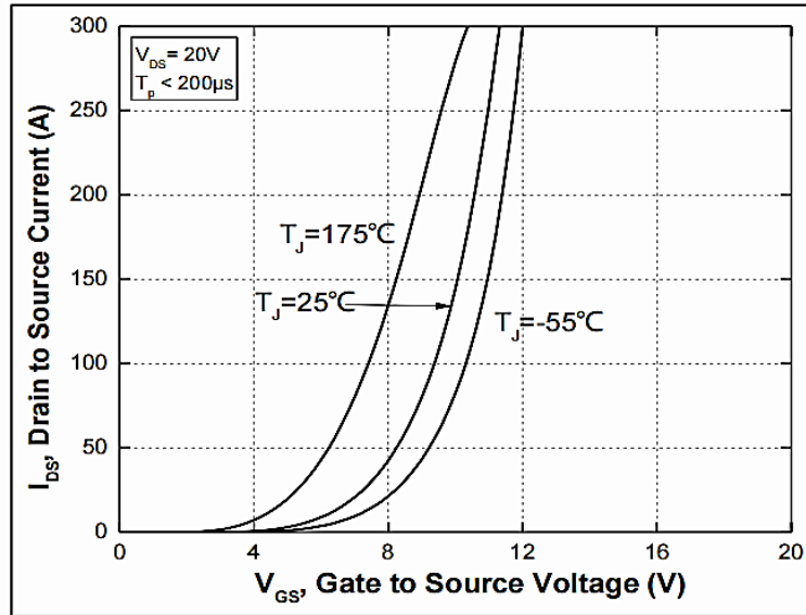
Figure 7. Transfer Characteristic for Various Junction Temperatures
