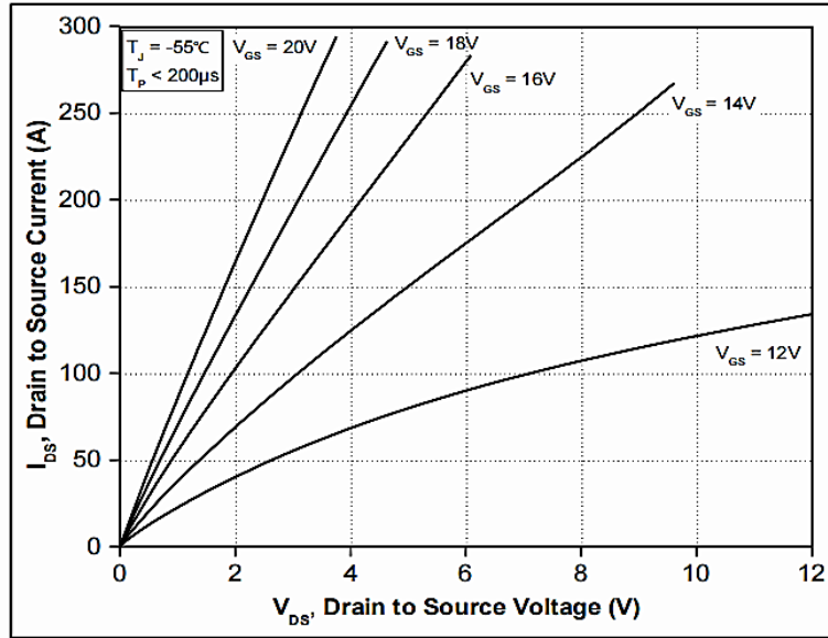
Figure 1. Output Characteristics T_J = -55^\circ\text{C}
