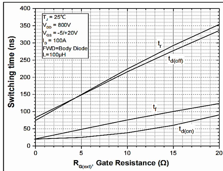
Figure 26. Switching Time vs. R_{G(ext)}
