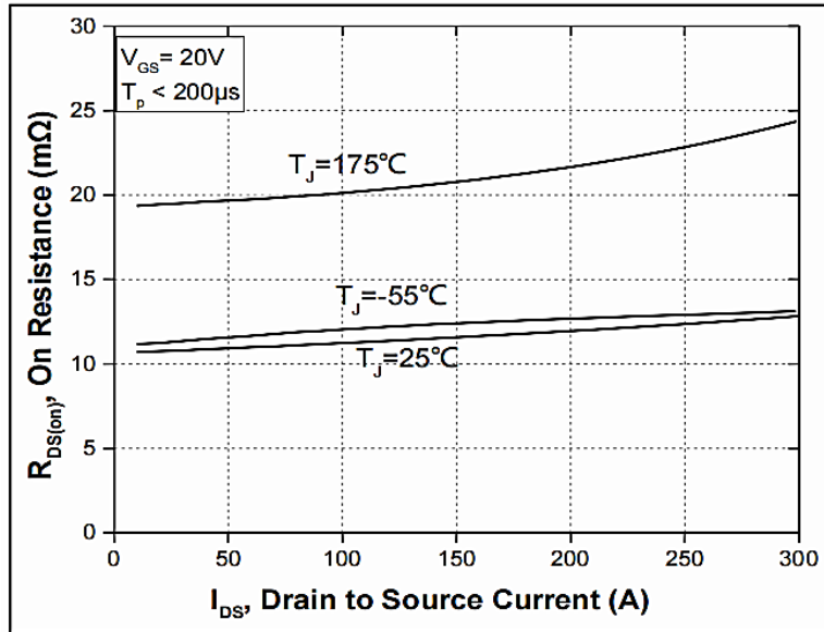
Figure 5. On-Resistance vs. Drain Current For Various Temperatures
