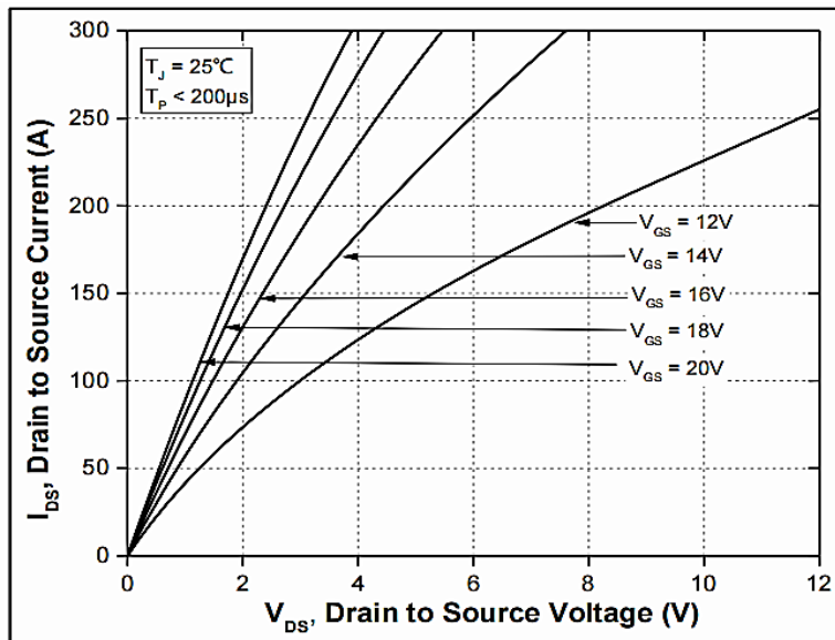
Figure 2. Output Characteristics T_J = 25^\circ\text{C}
