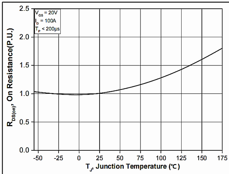
Figure 4. Normalized On-Resistance vs. Temperature
