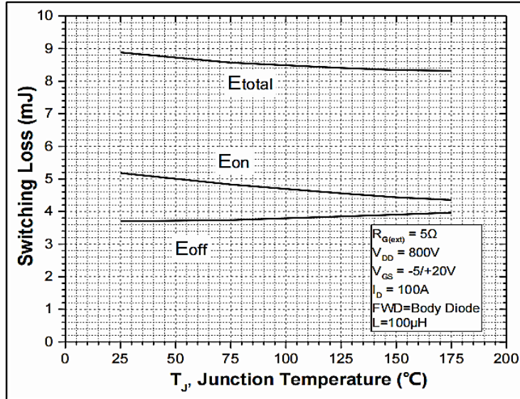
Figure 25. Clamped Inductive Switching Energy vs. T_j
