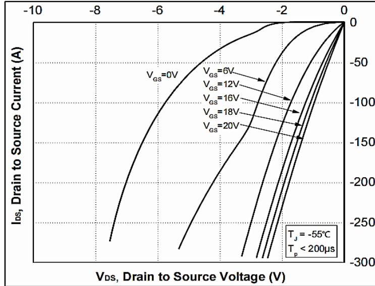
Figure 13. 3 rd Quadrant Characteristic at -55^{\circ}\text{C}
