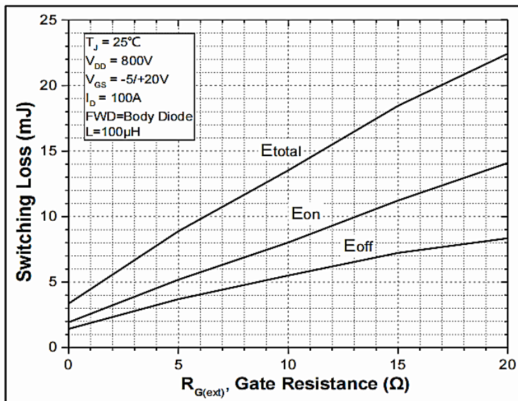
Figure 24. Clamped Inductive Switching Energy vs. R_{G(ext)}
