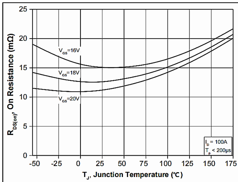
Figure 6. On-Resistance vs. Temperature For Various Gate Voltage
