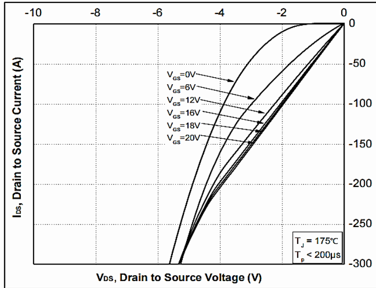
Figure 15. 3 rd Quadrant Characteristic at 175°C
