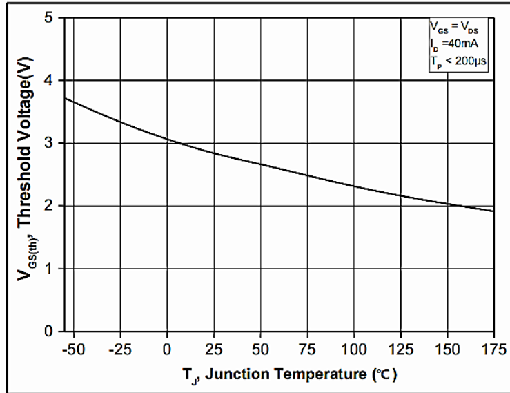
Figure 11. Threshold Voltage vs. Temperature
