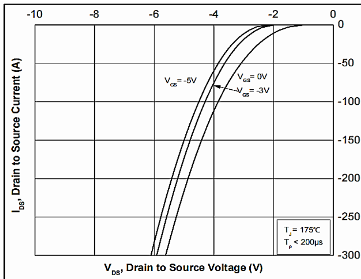
Figure 10. Body Diode Characteristic at 175°C
