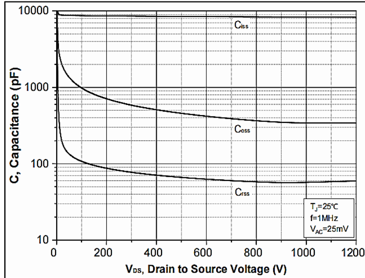
Figure 17. Capacitances vs. Drain-Source Voltage
