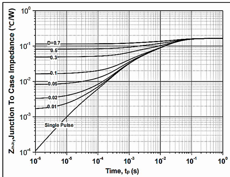
Figure 20. Transient Thermal Impedance (Junction - Case)
