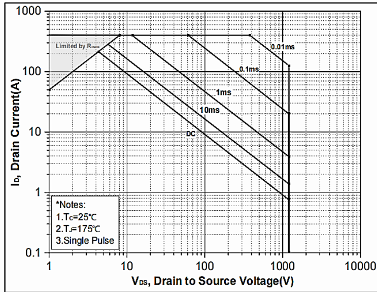
Figure 21. Safe Operating Area
