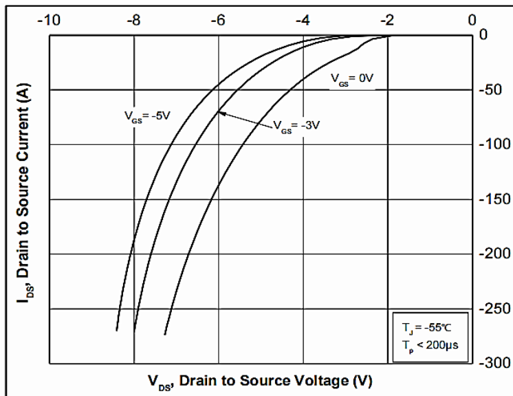
Figure 8. Body Diode Characteristic at -55°C
