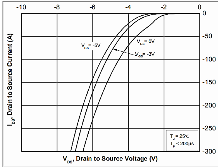
Figure 9. Body Diode Characteristic at 25°C
