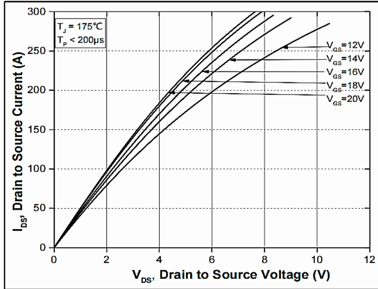
Figure 3. Output Characteristics T_J=175^\circ\text{C}
