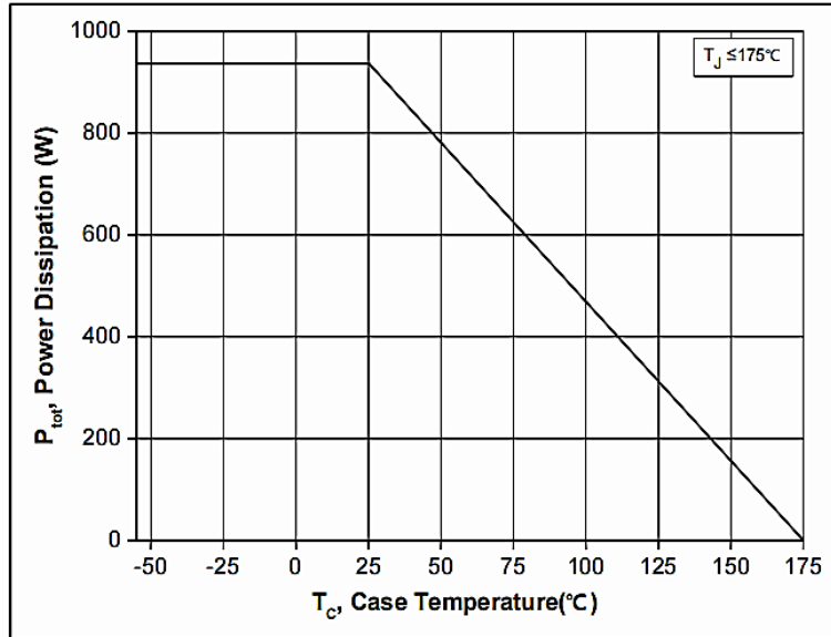
Figure 19. Maximum Power Dissipation Derating vs. Case Temperature
