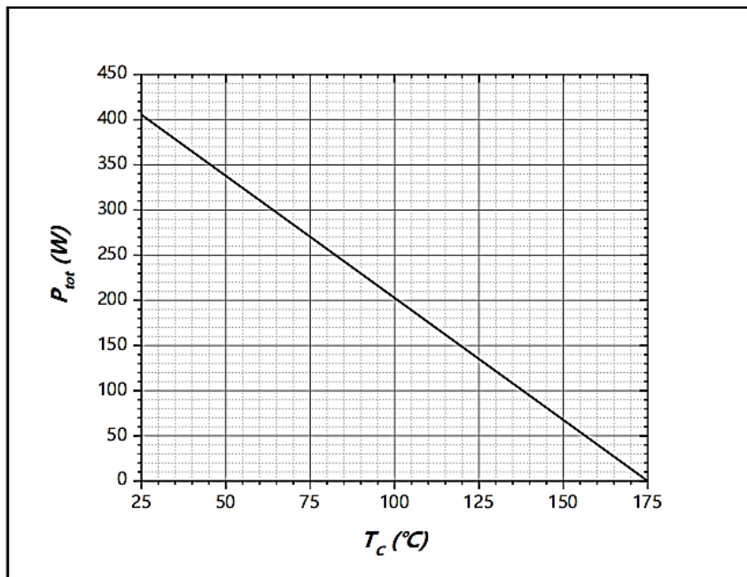
Figure 4. Power Derating
