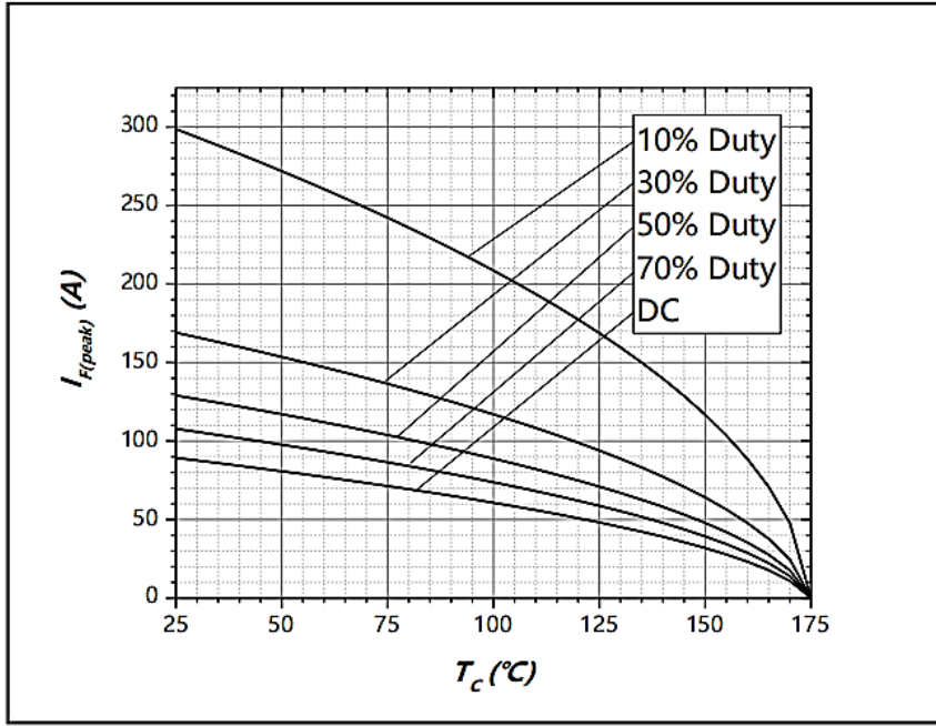
Figure 3. Current Derating
