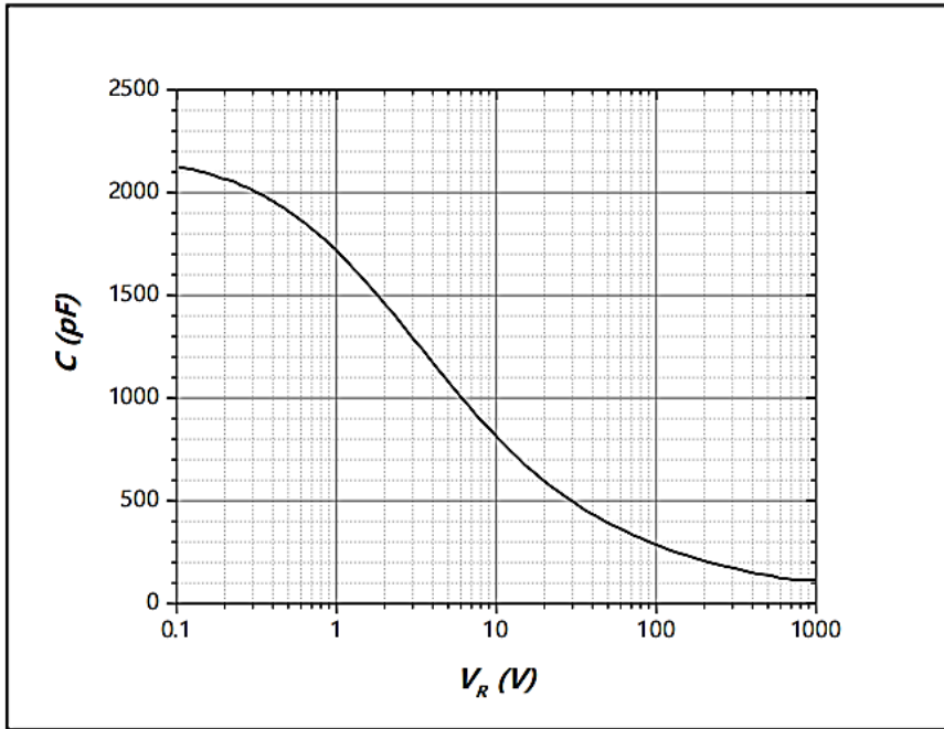
Figure 5. Capacitance vs. Reverse Voltage
