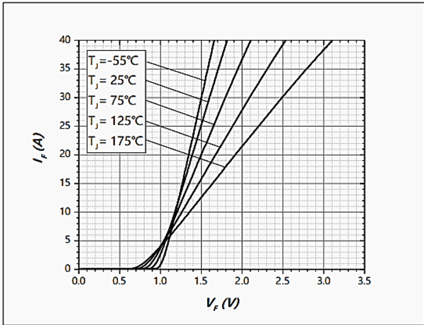
Figure 1. Forward Characteristics
