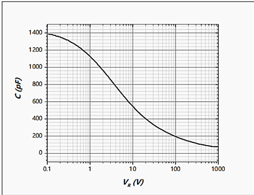
Figure 5. Capacitance vs. Reverse Voltage
