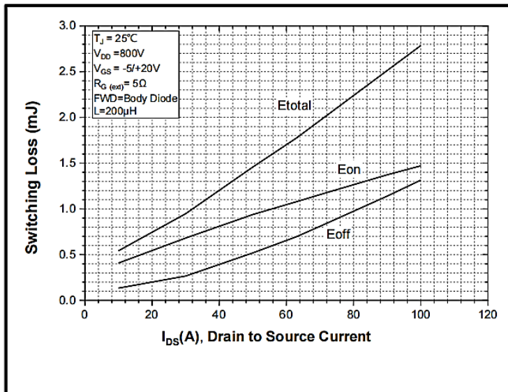
Figure 24. Clamped Inductive Switching Energy vs. Drain Current ( V_{DD}=800V , R_{G(ext)}=5\Omega )
