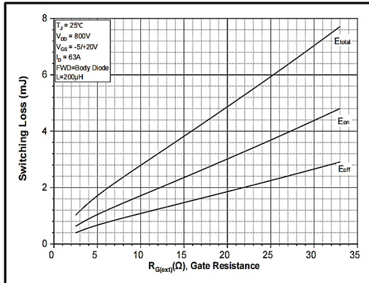
Figure 25. Clamped Inductive Switching Energy vs. R_{G(ext)}
