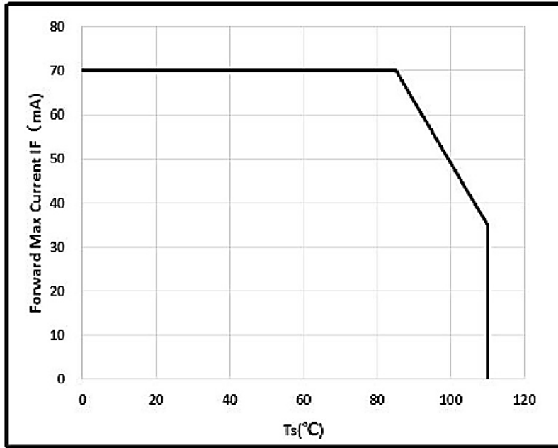
Figure 7 Ts Vs. Max. Permissible IF, I_F = f(T_s)
