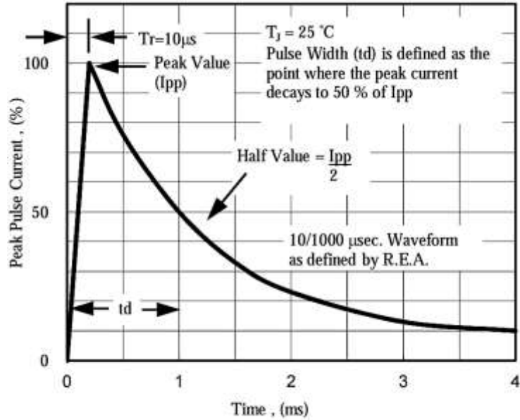
Fig. 5 - Pulse Waveform
