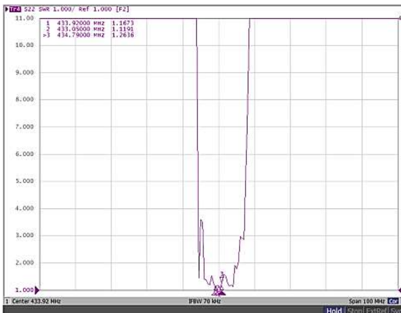
S22 VSWR
