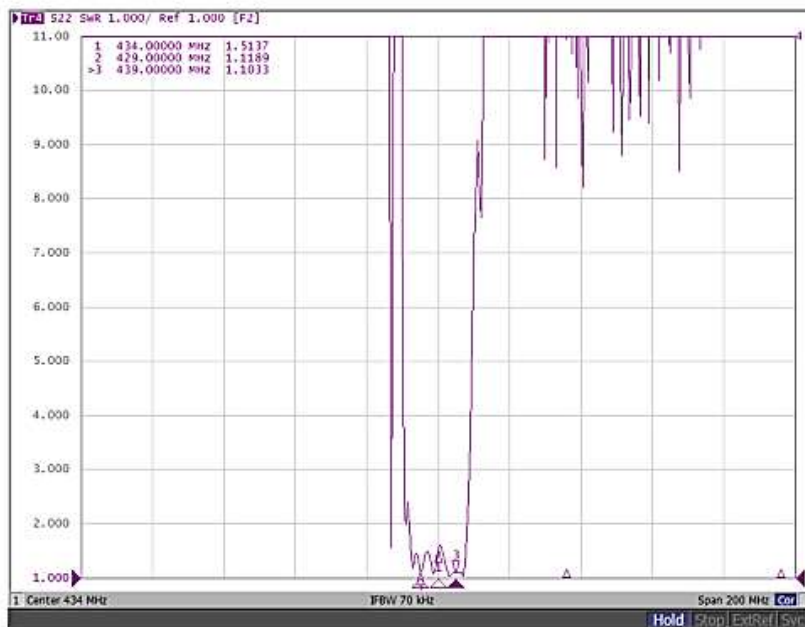
S22 VSWR
