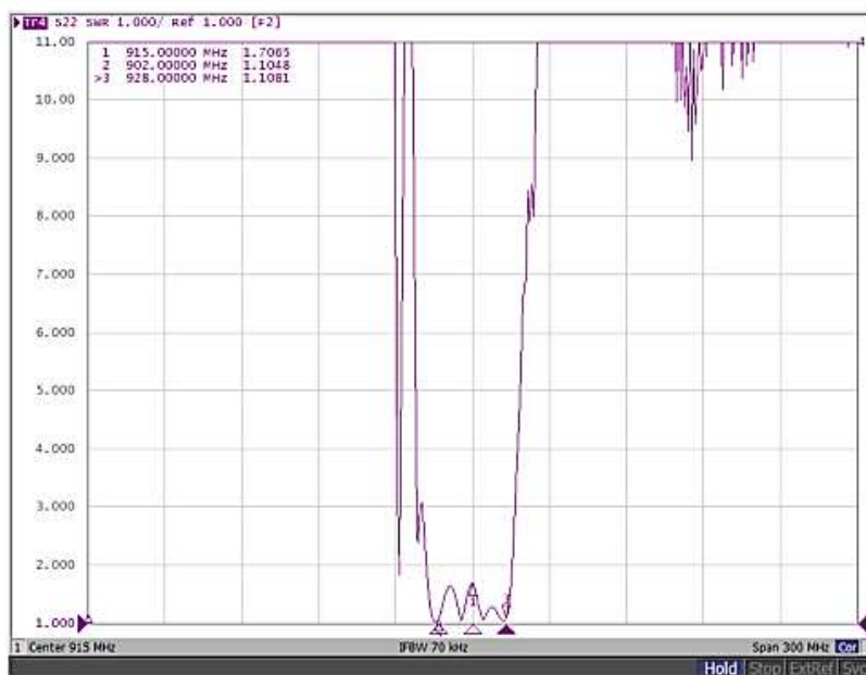
S22 VSWR
