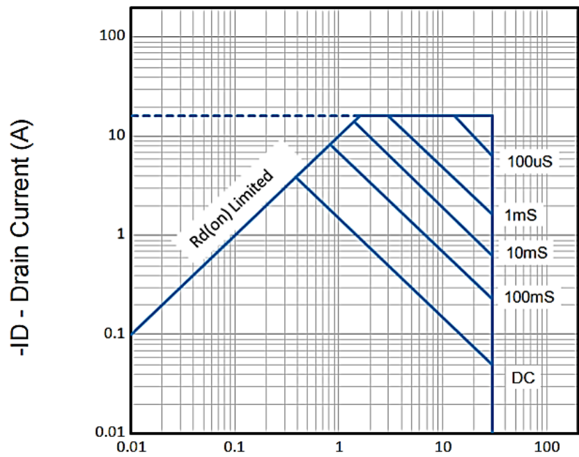
Figure 6. Maximum Safe Operating Area
