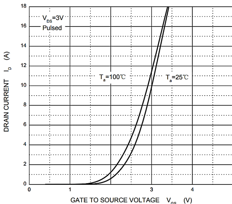
Figure 3. Typical Transfer Characteristics
