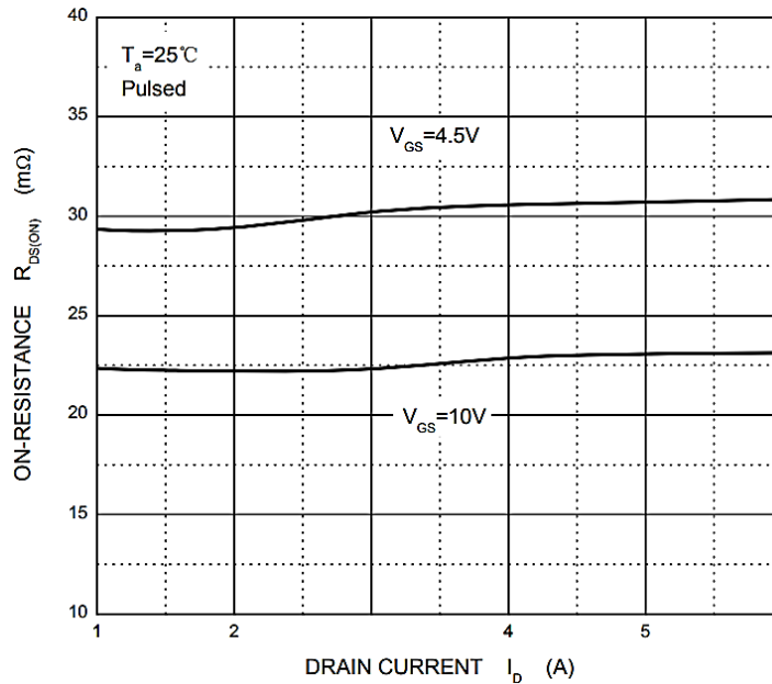
Figure 7. On Resistance R DS(ON) Vs. Drain Current I D
