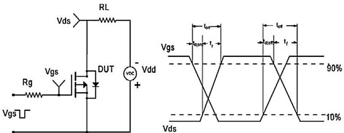
Figure 10. Switching Time Test Circuit and waveforms
