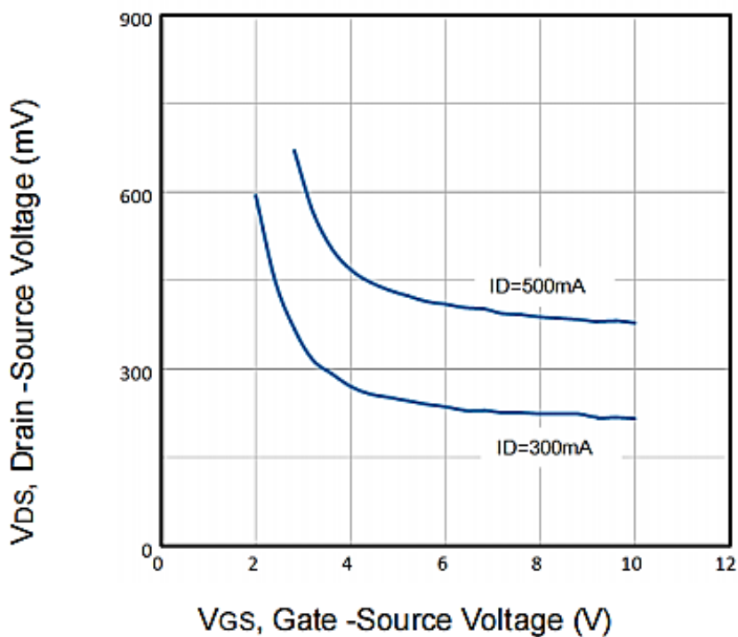
Figure 4. Drain -Source Voltage vs Gate -Source Voltage
