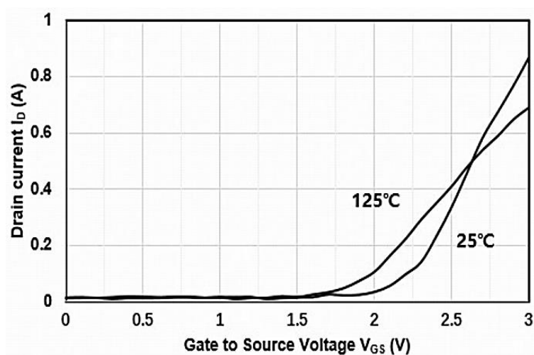
Figure 3. Transfer Characteristics
