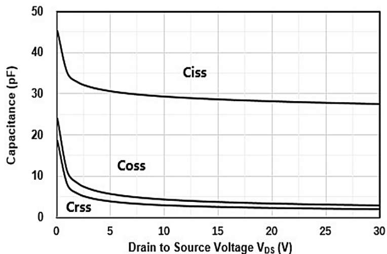
Figure 5. Capacitance Vs. Drain-Source Voltage
