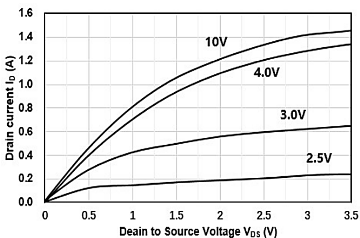
Figure 1. Output Characteristics
