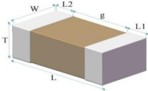
Fig.1: Structure & Dimension
