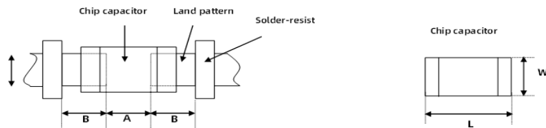
Recommended land dimensions for reflow-soldering
