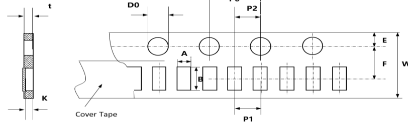
Fig. 5-4 0105, 0201 (Paper tape/ 2 mm pitch)
