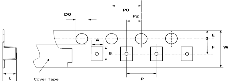
Fig. 5-2 0603,0805,1206,1210 (Plastic tape)
