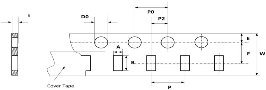
Fig. 5-1 0603, 0805, 1206, 1210 (Paper tape)
