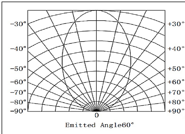
Figure 8. Radiation Diagram, I rel = f (Φ)
