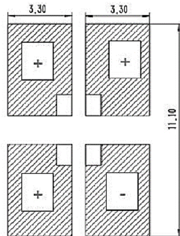
Recommended Stencil opening
