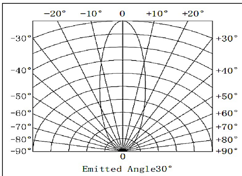
Figure 8. Radiation Diagram, I_{rel} = f(\Phi)
