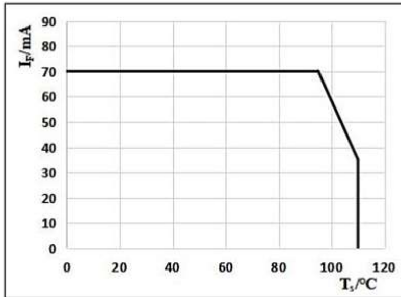
Figure 7 Ts Vs. Max. Permissible IF, I_F = f(T_s)
