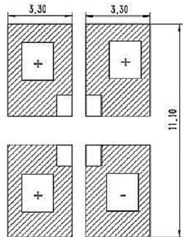
Recommended Stencil opening
