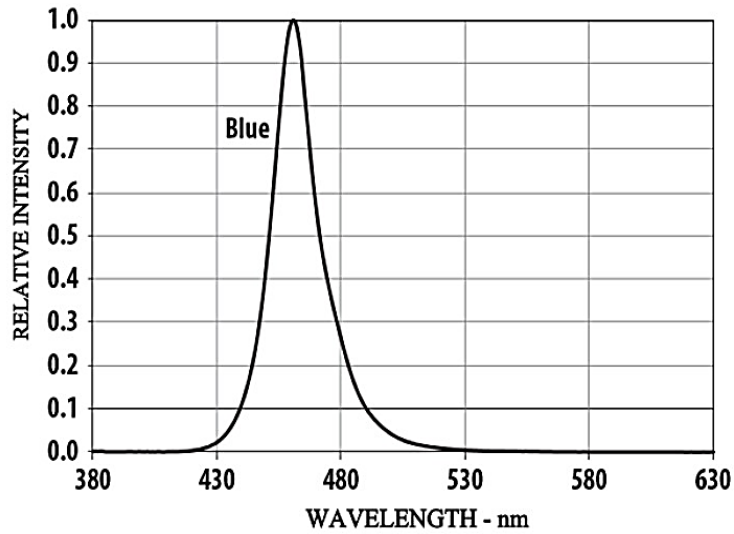
Figure 1. Relative Intensity vs. Wavelength
