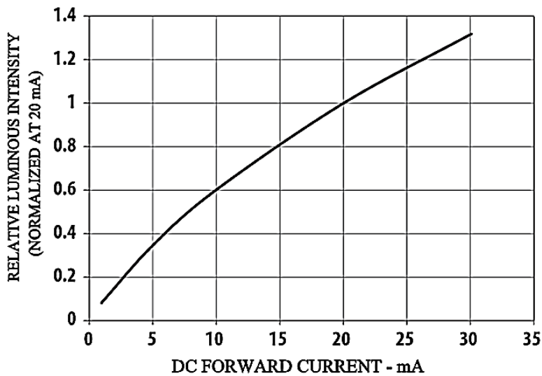
Figure 2. Relative Intensity vs. Forward Current
