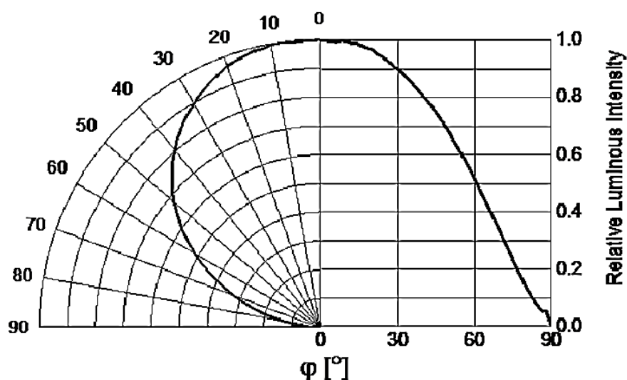
Figure 8. Representative Radiation Pattern for 120°, Viewing Angle Lamp
