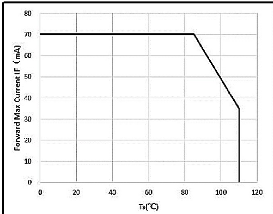
Figure 7 T_s Vs. Max. Permissible I_F , I_F = f(T_s)
