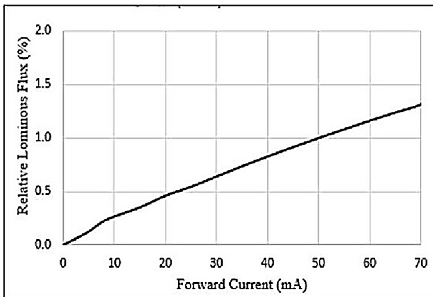
Figure 2. Forward Current Vs. Relative Intensity, \Phi_V/\Phi_V(50mA)=f(I_F)
