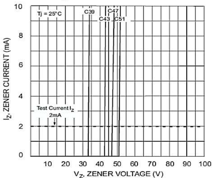
Fig. 4 Zener Breakdown Characteristics
