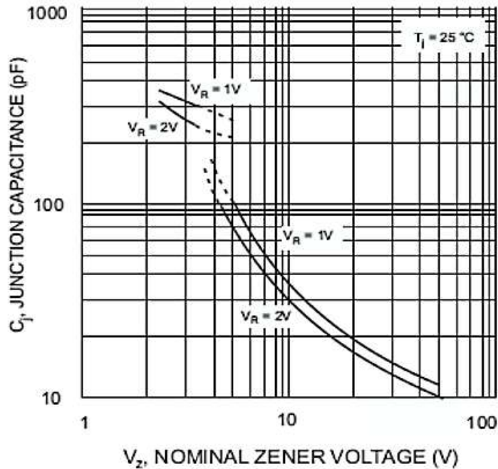
Fig. 5 Junction Capacitance vs Nominal Zener Voltage
