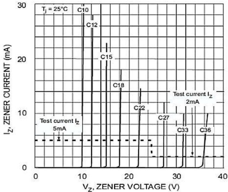
Fig. 3 Zener Breakdown Characteristics
