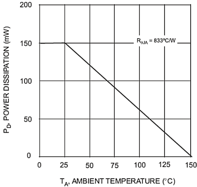
Fig. 1 Derating Curve
